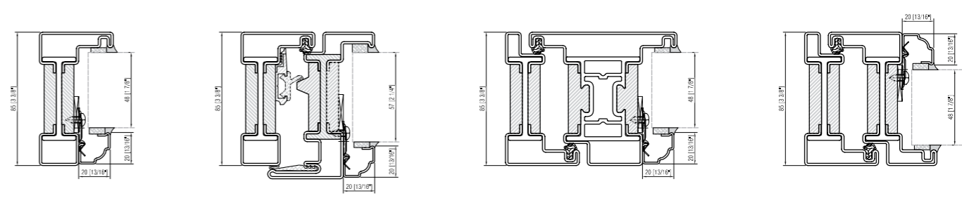
WINDOW open in interior glazing bead
