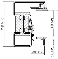
FIXED FRAME interior glazing bead
