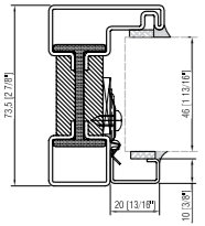
FIXED FRAME interior glazing bead
