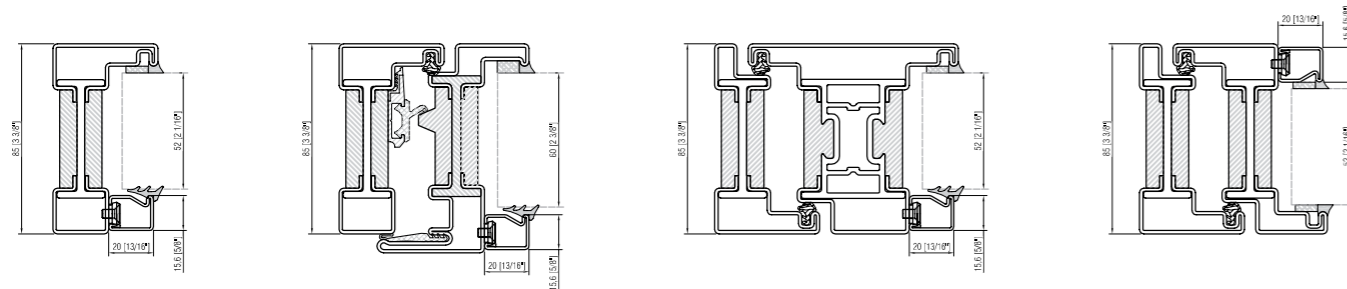
WINDOW open in interior glazing bead
