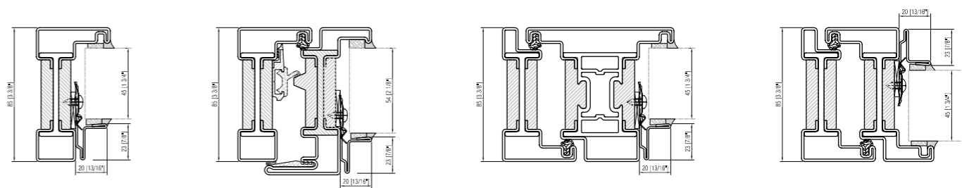
WINDOW open in interior glazing bead
