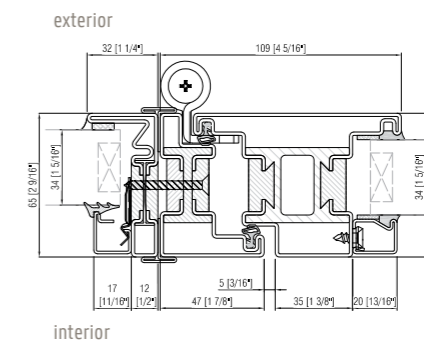
OS2 FXD mullered to EBE Hinged Door
