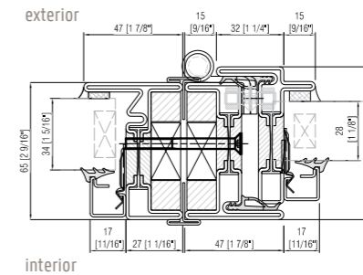
OS2 FXD mullered to OS2 CSMT with structural support inside the profile
