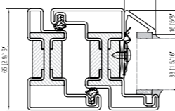
WINDOW open out exterior glazing bead
