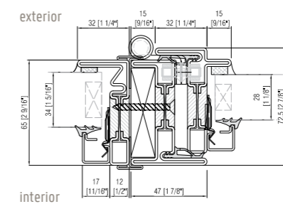
OS2 FXD mullered to OS2 CSMT Outswing
