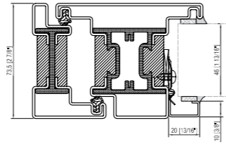
DOOR open out interior glazing bead
