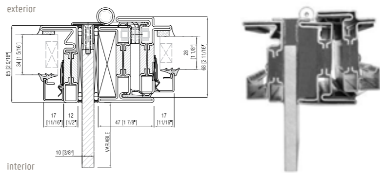
OS2 FXD muller to OS2 CSMT with structural 3/8" stiffener
