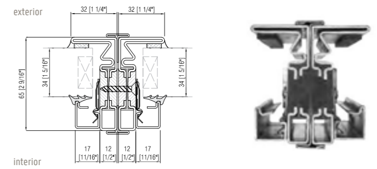
OS2 FXD direct muller to OS2 FXD
