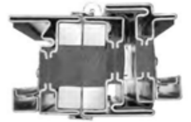
OS2 FXD mullered to OS2 CSMT with structural support inside the profile
