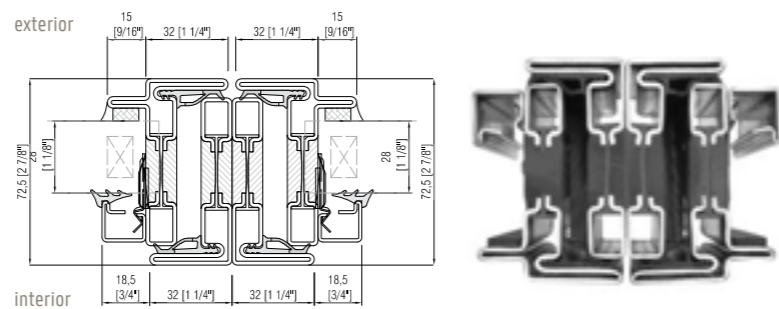
OS2 CSMT direct muller to OS2 CSMT
