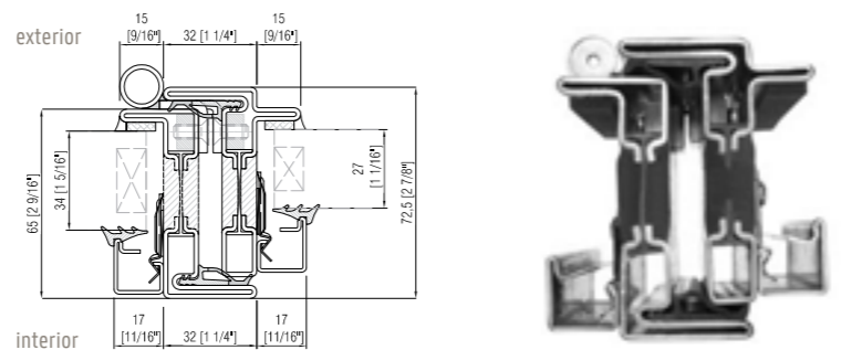
OS2 common frame FXD and CSMT
