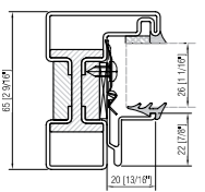
FIXED FRAME interior glazing bead
